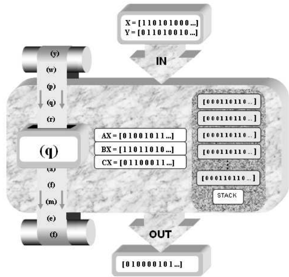
Fig. 1. The digital organism used by Avida, similar to that shown in the original Avida paper [16]. Generating a program from a fixed alphabet of 26 instructions (see Table I ) to perform a specified function like XNOR (EQU) is similar to generating a specified word or phrase from the English alphabet somewhere within an alphabet of characters. The Avida simulation actually make use of three inputs, X, Y and Z, in a circular queue. Whenever an input is read by the program, it is removed from the queue and then placed at the back of the queue. As a result, three consecutive reads will read in three different inputs, whereas the fourth will read the first input in again. This property was not addressed in the original paper.
