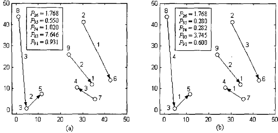
Fig. 4. Slot schedules obtained using (a) the per-frame model and (b) the per-slot model. \mu = 0.001 was used for both models. The per-frame model uses 3 slots to accommodate all requests but the per-slot model uses 4 slots. The numbers above the directed edges represent the slots to which the requests have been assigned. Because the per-slot model uses one more time slot, its total transmit power cost (6.675 units) is smaller than the total transmit power cost of the per-frame model (11.915 units).
