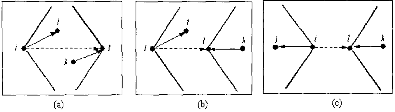
Fig. 1. Illustrating the effect of sectoring on interference power. Let G_{il} = s_{il}d_{il}^{-\alpha} be the link gain from node i to node l . Assume that the F/B ratio of all nodes is 20dB. (a) Consider the effect of the transmission i \rightarrow j , at a power level P_{ij} , on receiver l . Note that nodes i and k are located in the same sector with respect to node l . Also, nodes j and l are located in the same sector with respect to node i . In this scenario, the mainlobe of l is directed towards k and i , and the mainlobe of i is directed towards j and l . Consequently, the interference power at node l is equal to: P_{ij}S^2G_{il} . (b) In this figure, while the mainlobe of node i is still directed towards j and l , node l 's backlobe is directed towards i . Since an F/B ratio of 20dB corresponds to a backlobe gain of 1/100^{th} the mainlobe gain, the interference power at node l in this case is equal to: P_{ij} \left( \frac{S^2}{100} \right) G_{il} . (c) In this figure, the backlobe of node i is directed towards l and vice versa. Consequently, the interference power at node l is equal to: P_{ij} \left( \frac{S^2}{10000} \right) G_{il} .
