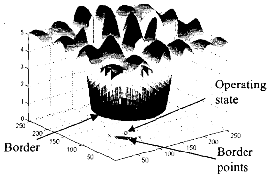
Fig.5. Example of contour identification where points are distributed relatively uniformly on the contour and close to the operating state.
